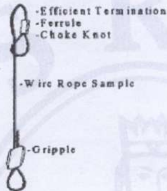
Test configuration
